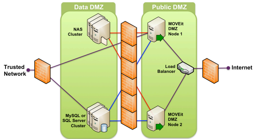
MOVEit DMZ Enterprise Two Node HA Web Farm Deployment
