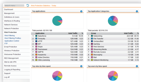
Top-Domain-Reporting
