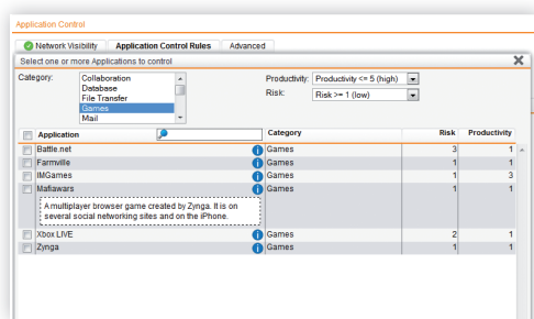
Application Control
